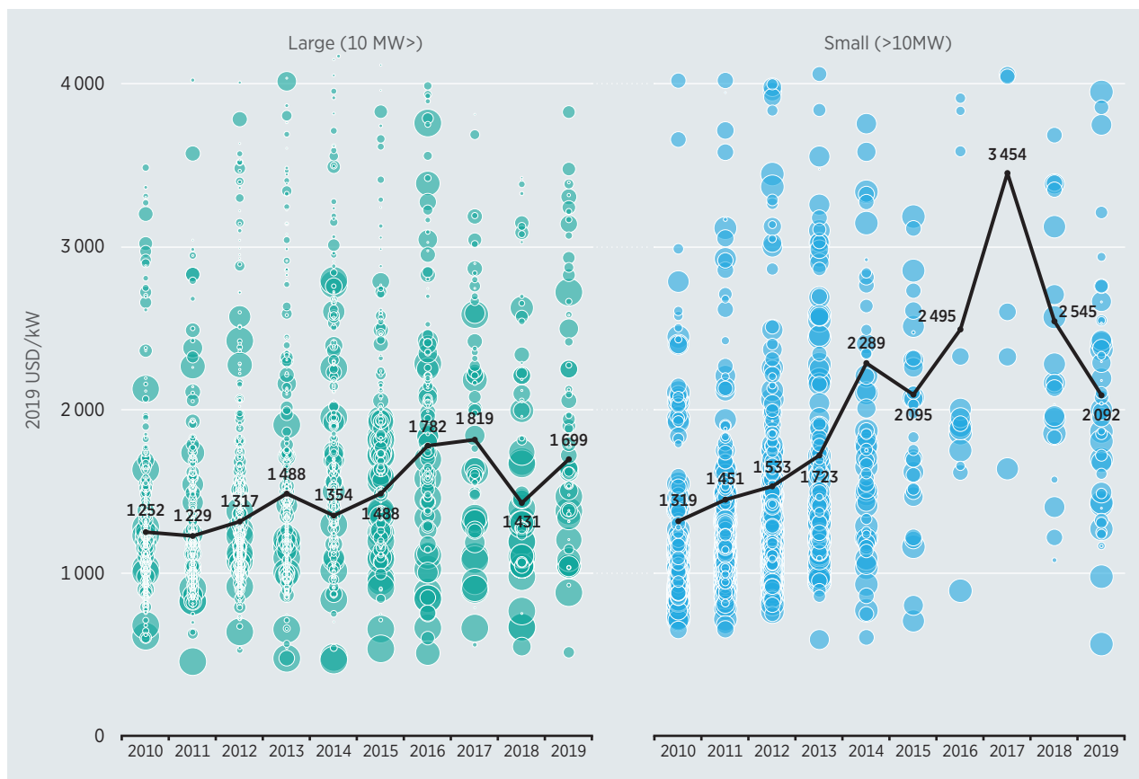
Figure 5.3 Total installed costs for small and large hydropower projects and the global weighted average, 2010-2019
