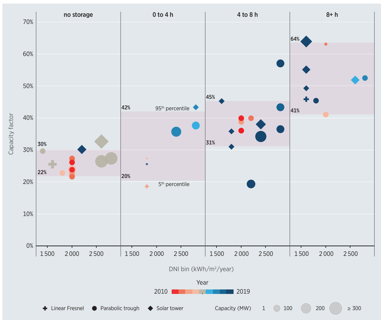
Figure 8.4 Capacity factor trends for CSP plants by direct normal irradiance, 2010-2019
